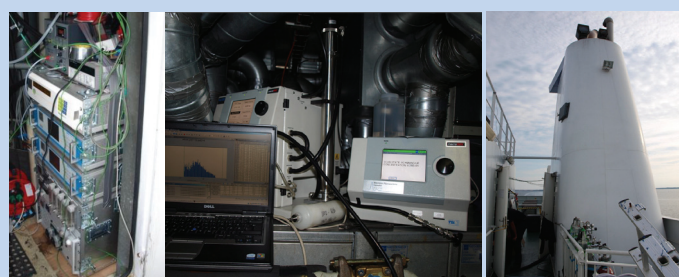
Figure 1: Experimental setup with measurement equipment and chimney
