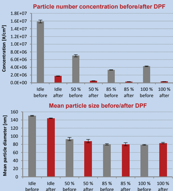
Figure 2: Particle number concentration and mean particle size for engine load: Idle, 50 %, 85 % and 100 % MCR, measured with SMPS during operation
